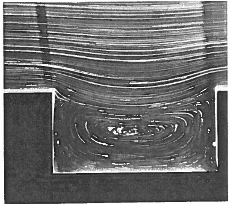
b/h=2
