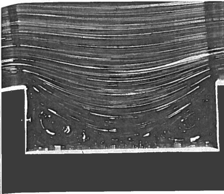
b/h=3
