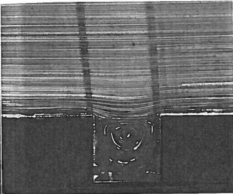
b/h=1
